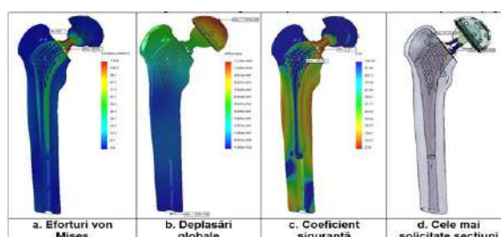
Advanced finite element analysis hip prosthesis
