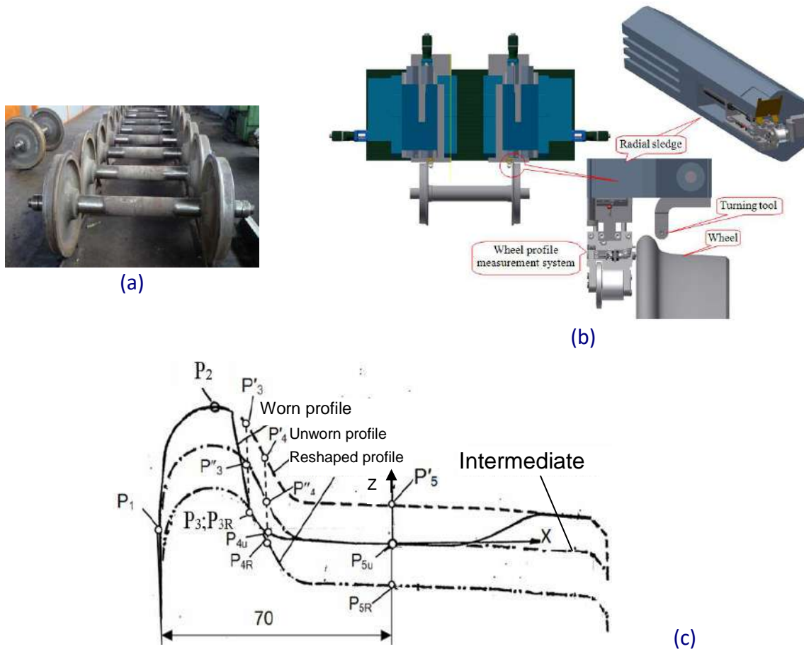
Figure 1.a. Wheelsets; b. Profile measurement system; c. Measurement points
