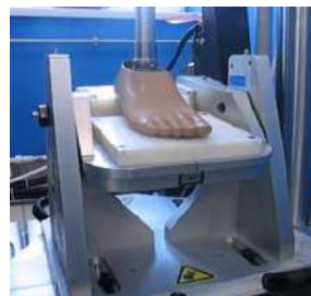
Test subassembly "ankle-foot prosthesis lower limb external"
