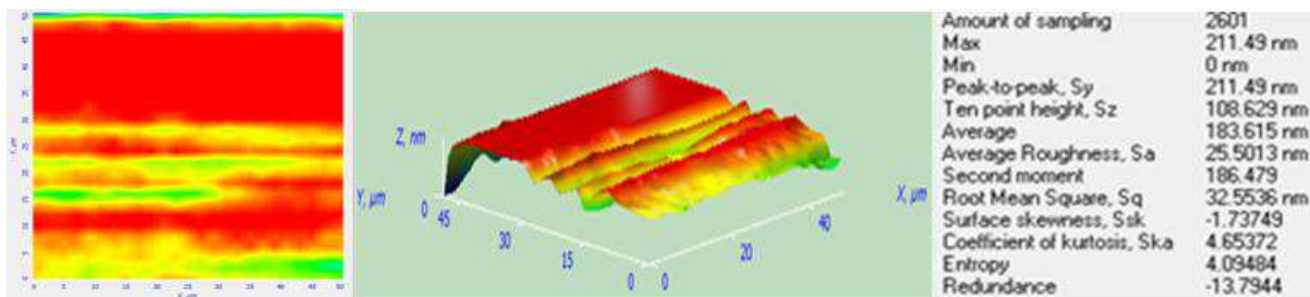
50 nm thick aluminium layer deposited on steel substrate type Rul.
