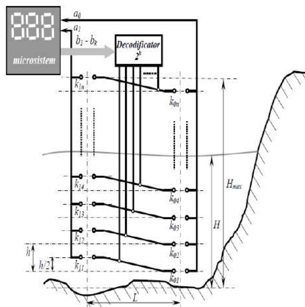
Fig.1 Scheme mounting sensors
