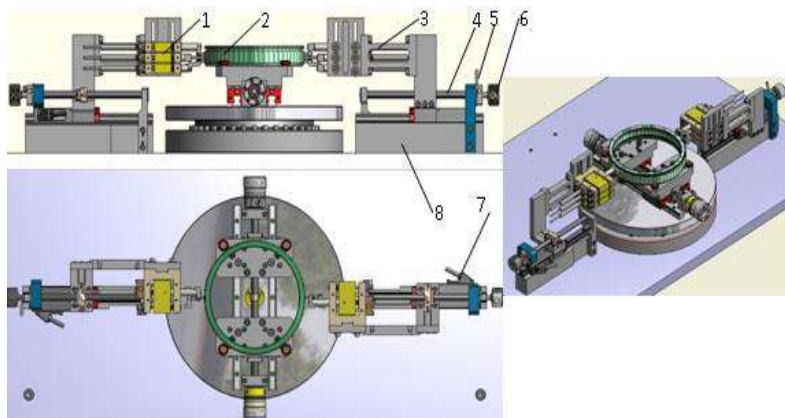
Figure 2 Ring centering and outer surfaces measurement subassembly
